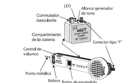
Fig. 1 - Controles
