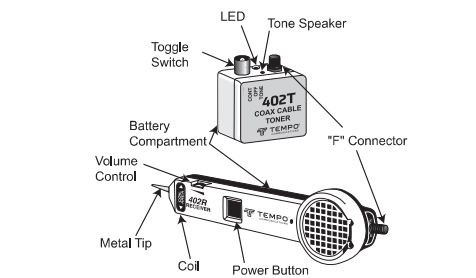
Fig. 1 - Controls
